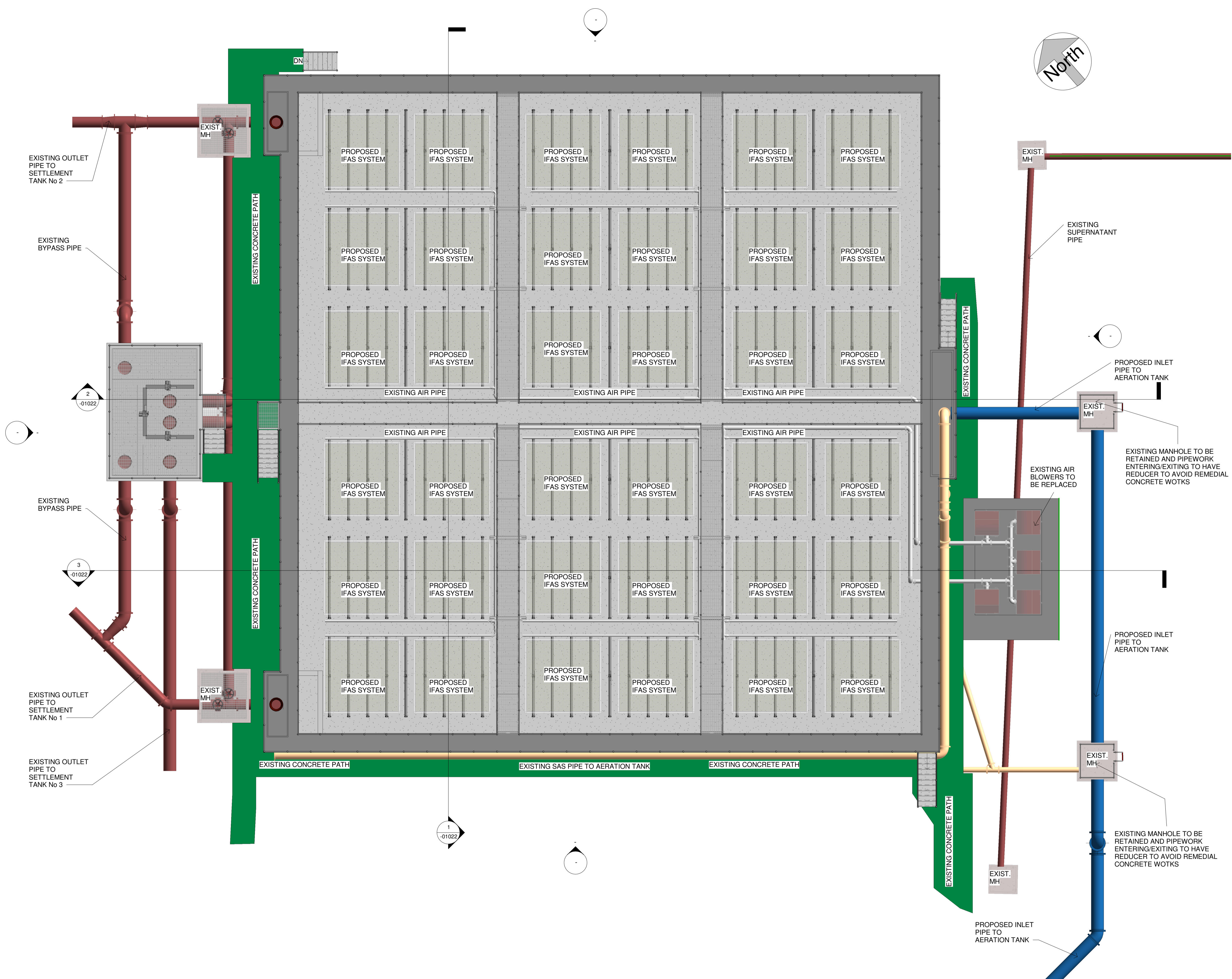
1 AERATION TANK @ FLOOR LEVEL 1 : 100
